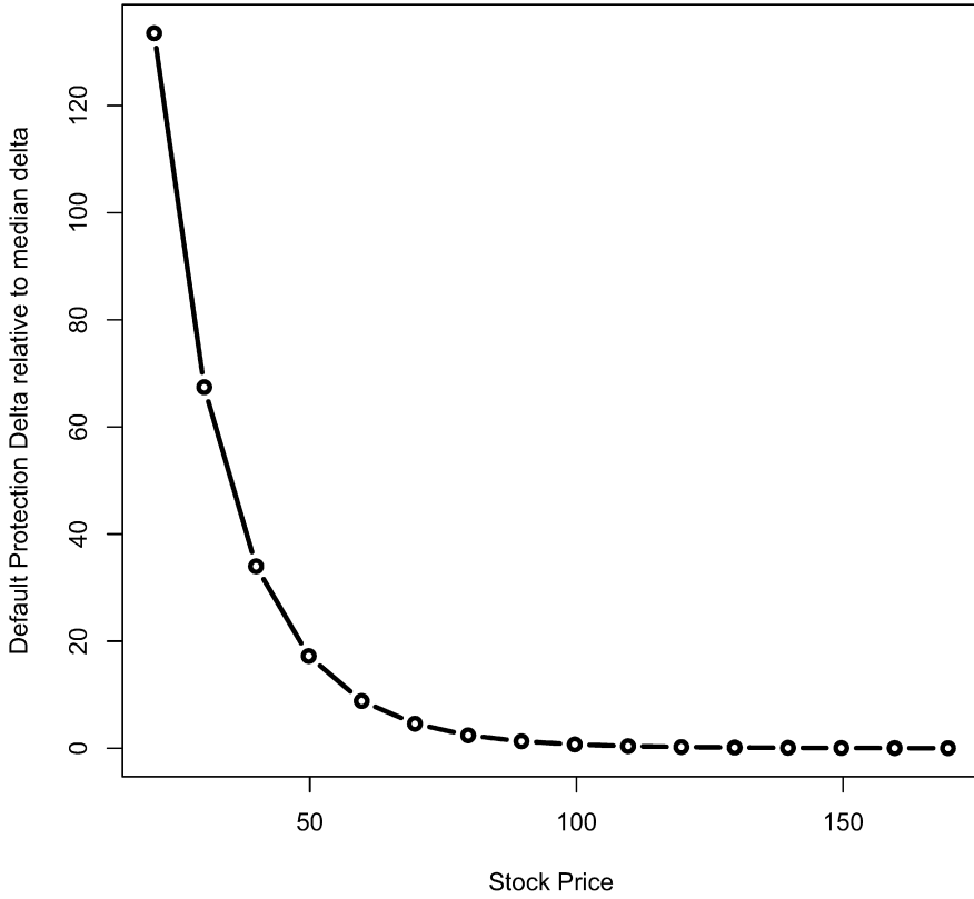
Fig. 1. Delta of the CDS. The plot shows how the delta of the CDS contract changes when the stock price changes. This plot was generated by varying firm value from 50 to 200, and computing the stock price and the delta of the CDS. We plot the delta divided by the median delta for this range of firm value, based on Eq. (5). The parameters of the Merton model were set to: debt face value F = 50 , debt maturity T = 5 years, risk-free rate r = 10\% , and firm asset volatility \sigma = 20\% . Since CDS hedging costs are proportional to the delta of the CDS with respect to the stock price, we see that delta increases rapidly as the stock price declines, implying that poor quality firms' CDS spreads will be more sensitive to equity market illiquidity.
